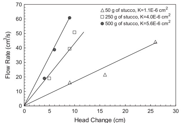
Fig. 4. Constant head permeability test results.
