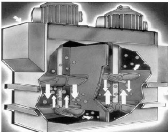
Figure 5: Attrition-scrubbing cells (Courtesy Metso Minerals)
