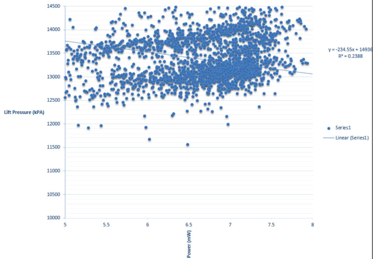
SAG 1 Load Curve for Jan 2020
